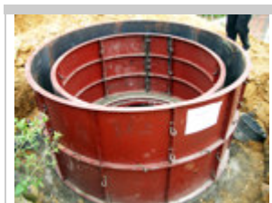
4. assemble the digester neck mould
